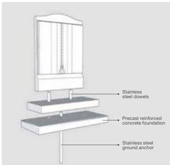
Ground Anchor Fixing Method
